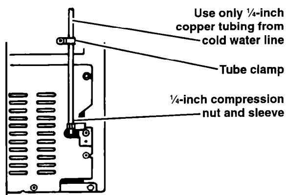
Style #2 valve
